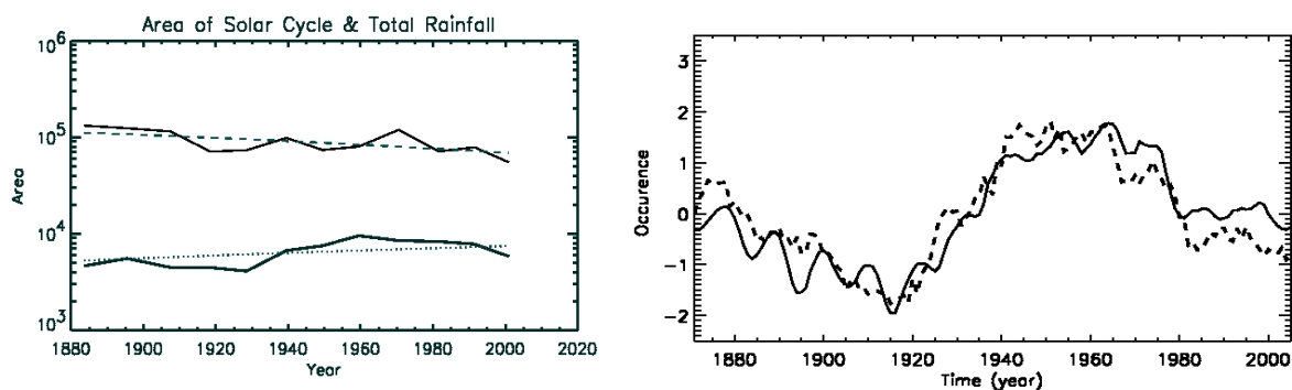
Fig 6. (a) The left figure represents the long term variation of the areas of sunspot (increasing trend) and the rainfall (decreasing trend) variabilities. The dotted and dashed lines are the linear least square fit to the respective data, (b) the right figure (by removing long term decreasing trend in the rainfall and increasing trend in the solar activity) illustrates the Indian Monsoon rainfall and sunspot activities. The continuous line is the occurrence of sunspot activity and dashed line is the rainfall variability.
