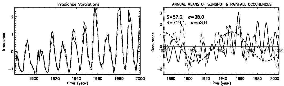
Fig 2. The deviation from the mean and normalized to their respective standard deviations of the annual solar and Indian rainfall occurrence variabilities. (a) In the left figure, the continuous line is the occurrence of sunspot number and the dotted line is irradiance variations, (b) In the right figure, the continuous line is sunspot occurrence variability and the dotted line is the annual Indian rainfall variability. The thick dashed curve is a long-term (~ 80-100 years) variation of the annual Indian rainfall variability. S and R are the means of the sunspot and rainfall occurrence variabilities. \sigma is the standard deviation from the mean of both the variabilities.
