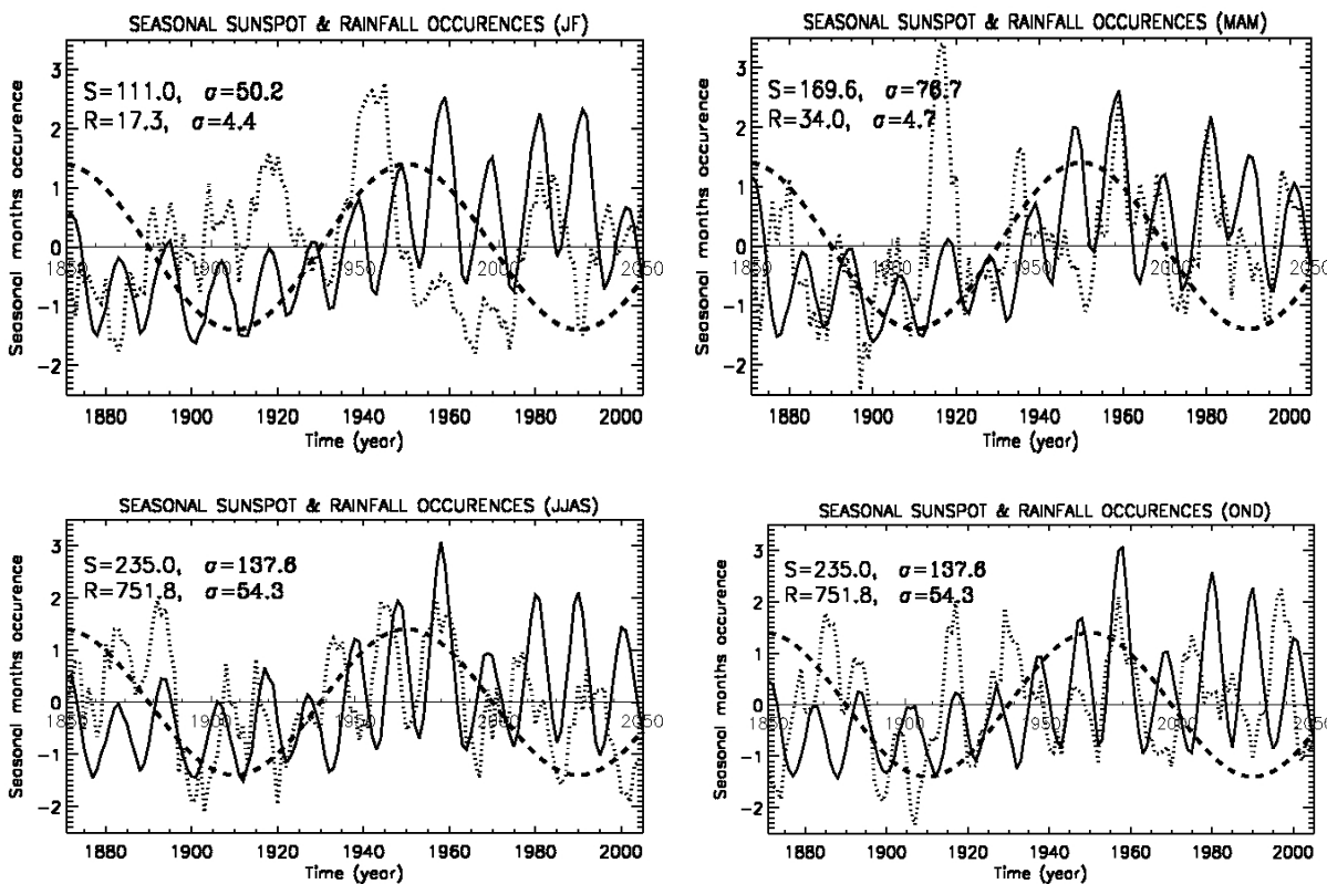
Fig 3. The deviation from the mean and normalized to their respective standard deviations of the seasonal sunspot (continuous lines) and Indian rainfall occurrence (dotted lines) variabilities. In all the above four figures, S is the mean of the sunspot activity, R is the mean of the rainfall variability and \sigma is the standard deviation from the mean for both the variabilities. The thick dashed curve is a long-term (~ 80-100 years) variation of the annual Indian rainfall variability.
