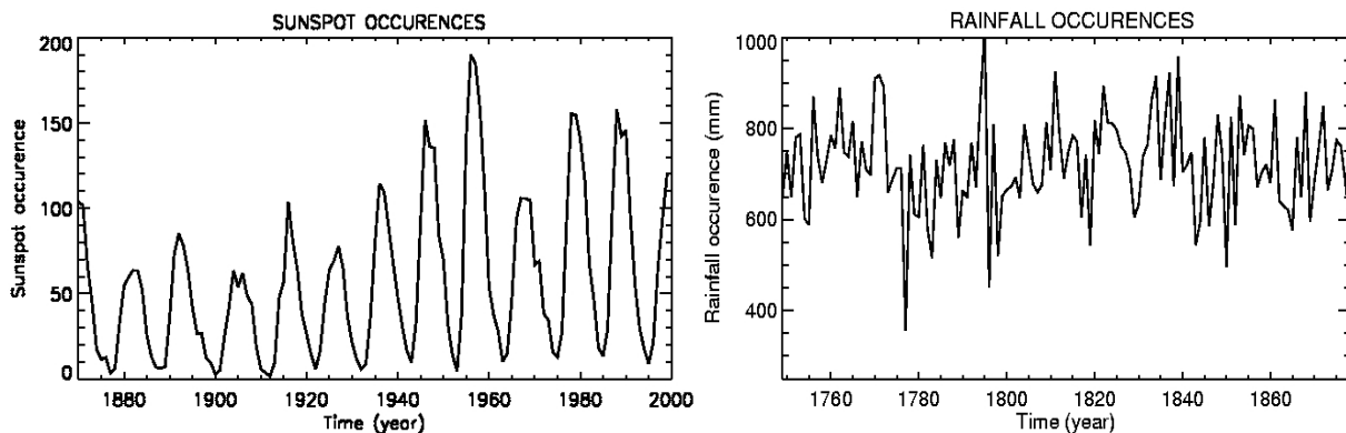
Fig 1 . (a) Temporal variation of the occurrence of the annual sunspot numbers. (b) Temporal variation of occurrence of the annual Indian rainfall.
