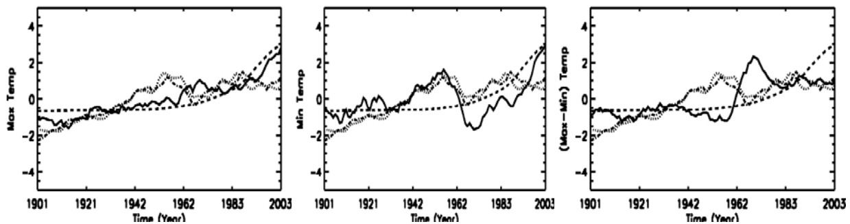
Fig 7. The deviation from the mean and normalized to the respective standard deviations of the temperature of the Indian subcontinent, Asian atmospheric concentration of carbon dioxide and solar activity variabilities. The continuous line is the surface temperature of the Indian subcontinent, the dashed line is the concentration of atmospheric carbon dioxide, the dotted line is the solar UV irradiance and the dash-dotted line is the geomagnetic aa index. All the three figures (fig 7(a), fig 7(b) and fig 7(c)) illustrate the maximum, minimum and the difference of maximum and minimum (maximum-minimum) temperature variabilities over plotted with the solar activity indices.
